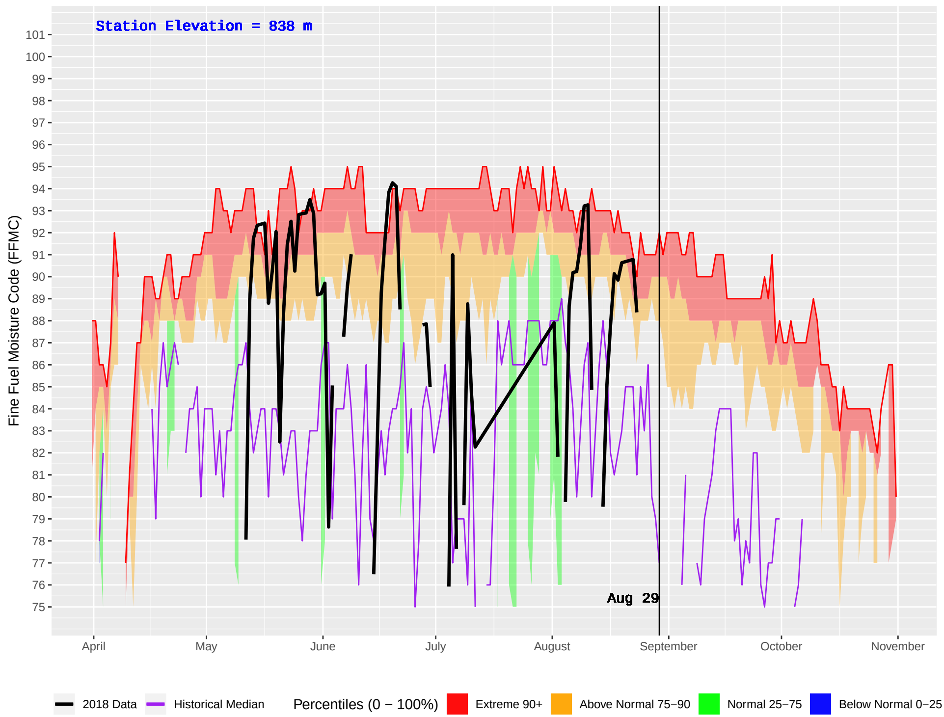
HOWARD (343) : Historical (1970–2016) and Current (2018) Daily Fine Fuel Moisture Code (FFMC)
